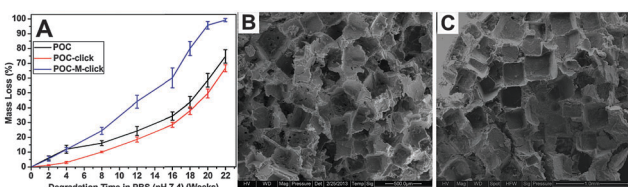
Fig. 3 (A) Degradation profiles of POC-M-click polymer films in PBS (pH 7.4) compared with POC and POC-click polymer films. All polymers were crosslinked at 100 °C for 3 days. Representative SEM images of POC-M-click–HA porous matchstick scaffold fabricated with (B) and without (C) using PVP for salt bonding.
