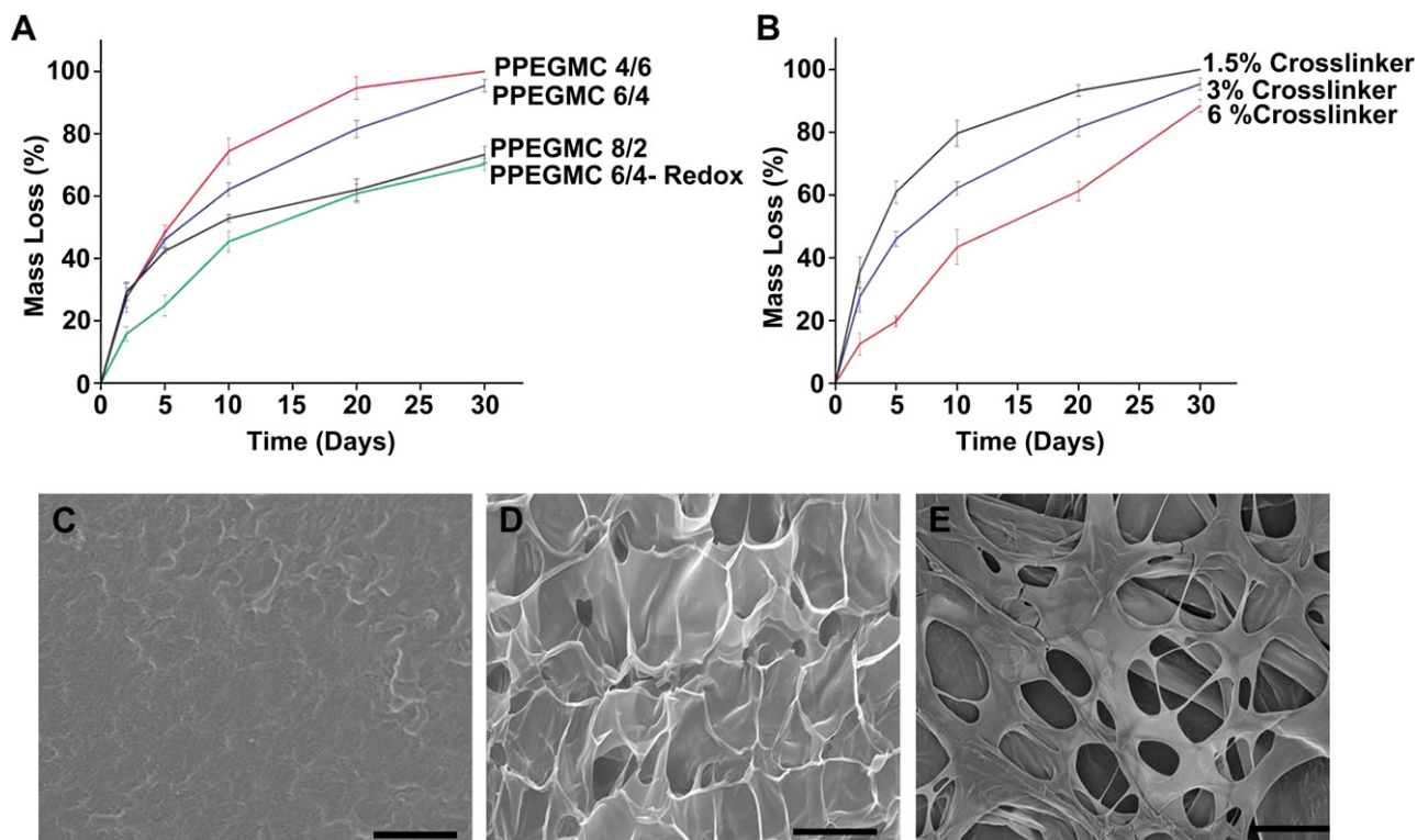
Fig. 6. In vitro degradation of PPEGMC. A) Mass loss of the photocrosslinked PPEGMCs and redox crosslinked (PPEGMC-Redox) hydrogels incubated in PBS (pH 7.4; 37 °C) for up to 30 days; B) Mass loss of the photocrosslinked PPEGMC6/4 crosslinked with 1.5, 3, and 6 v/v% of crosslinkers; SEM image of the degrading PPEGMC6/4 film at C) day 5, D) day 10, and E) day 20. PPEGMC exhibited smooth surface at day 5 and gradually turn into porous matrix over time. All scale bar = 200 \mu m.
