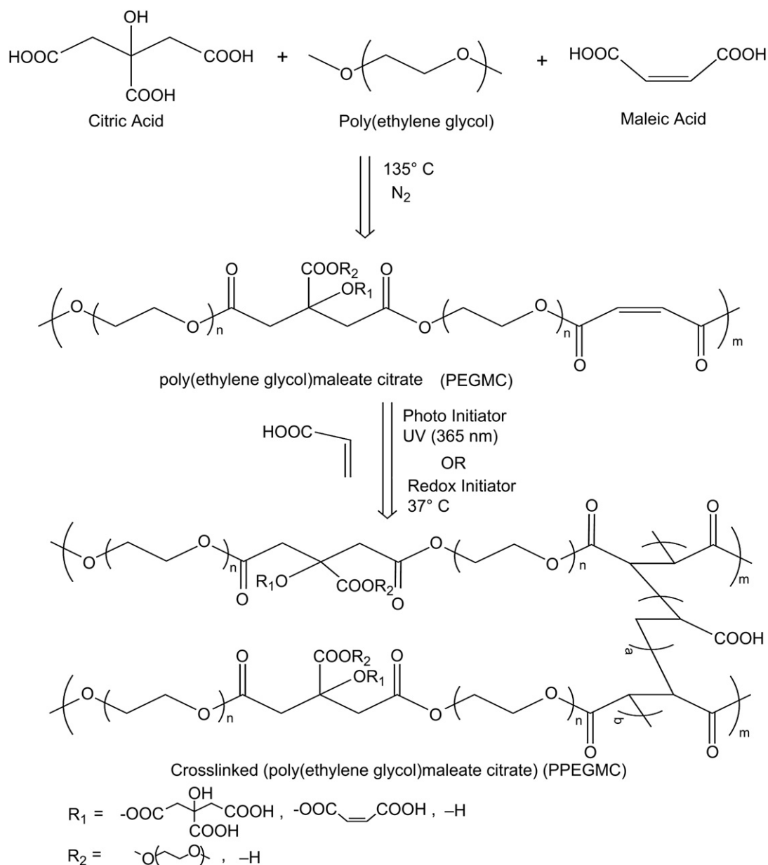
Fig. 1. Schematic representation of PPEGMC synthesis.
