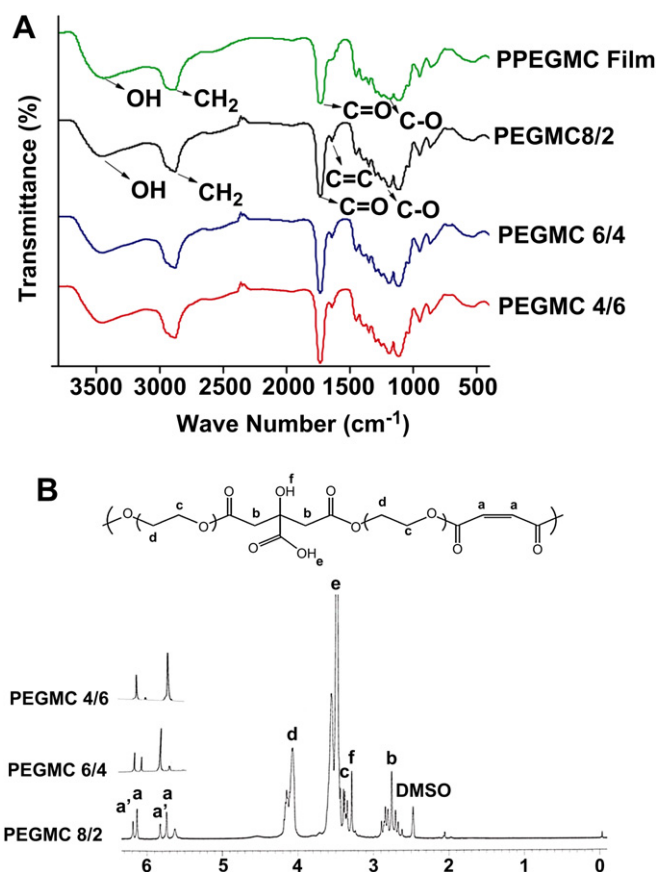
Fig. 2. Polymer Characterization of PEGMC. A) FTIR spectra of the PEGMC and the photocrosslinked PPEGMC; B) 1 H NMR spectrum of a representative PEGMC, PEGMC8/2.
