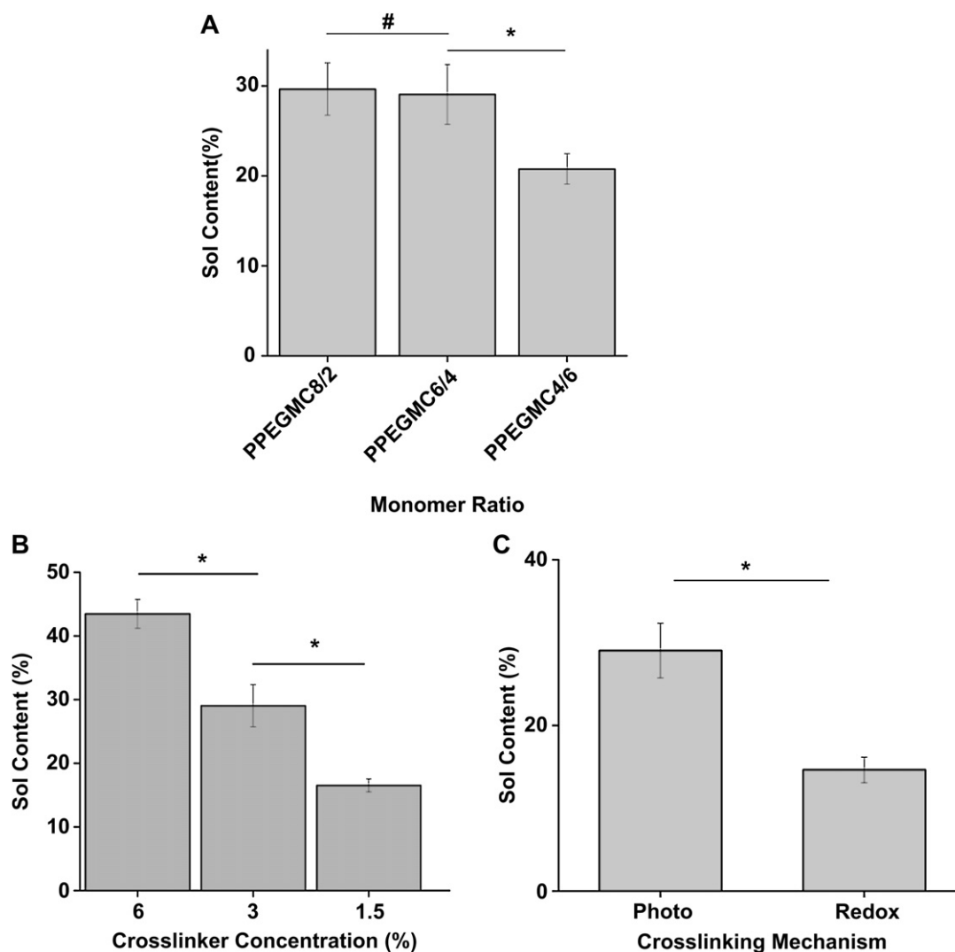
Fig. 3. Sol content of PPEGMC. A) Sol content of the PPEGMC8/2, PPEGMC6/4, and PPEGMC4/6 crosslinked with 3 v/v% of crosslinker and 0.11 M of photoinitiator for 1 min under UV radiation; B) Sol content of the PPEGMC6/4 crosslinked with 1.5 v/v%, 3 v/v%, and 6 v/v% of crosslinker and 0.11 M of photoinitiator for 1 min under UV radiation; C) Sol content of the PPEGMC6/4 initiated by photoinitiators and redox initiators (* p < 0.01 , # p > 0.01 ).
