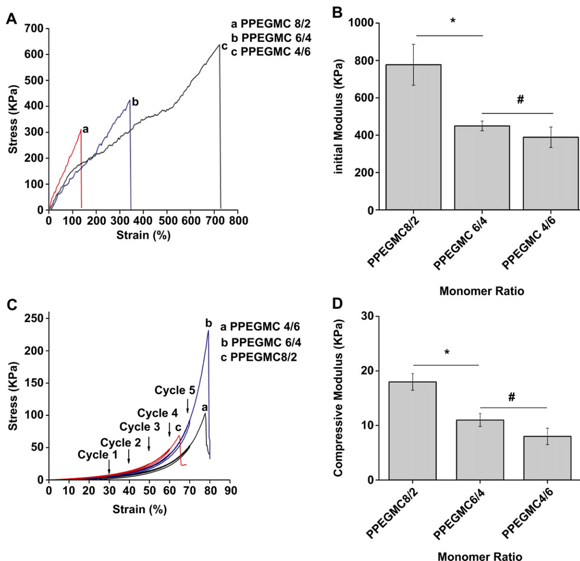
Fig. 5. Mechanical Properties of PPEGMC. A) Tensile stress–strain curve, B) initial modulus, and C) cyclic compressive stress–strain curve of the photocrosslinked PPEGMC8/2, PPEGMC6/4, and PPEGMC4/6; All the above PPEGMCs were crosslinked with 3 v/v% of crosslinker and 0.11 M of photoinitiator for 1 min under UV radiation; D) Initial modulus of the hydrated redox crosslinked PPEGMC8/2, PPEGMC6/4, and PPEGMC4/6 under the cyclic compressive tests. PPEGMCs were crosslinked with 3 v/v% of crosslinker, 0.026 M of APS and 0.11 M of TEMED for 1 min at 37 °C (* p < 0.01 , # p > 0.01 ).
